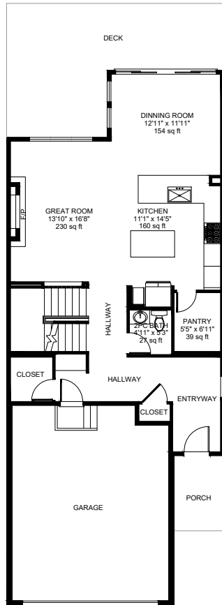
Main Floor Exterior Area: 993 sq ft
